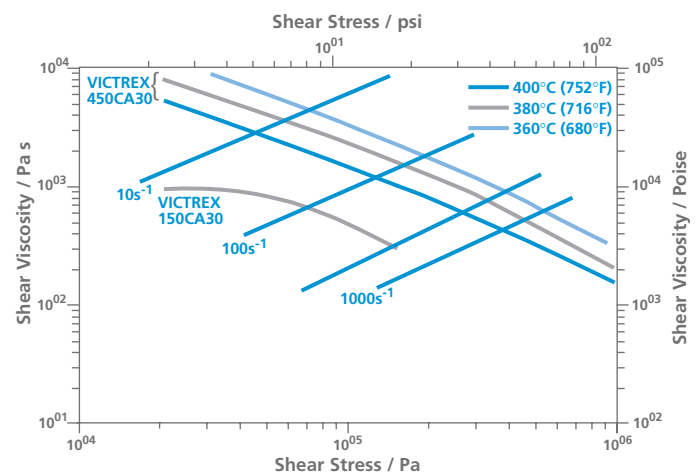
Figure 4: Shear Viscosity Versus Shear Stress for 30% Carbon Fiber Filled VICTREX PEEK
