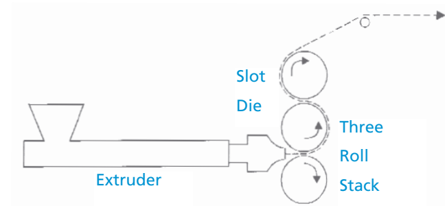
Figure 7: Sheet Producing Equipment
