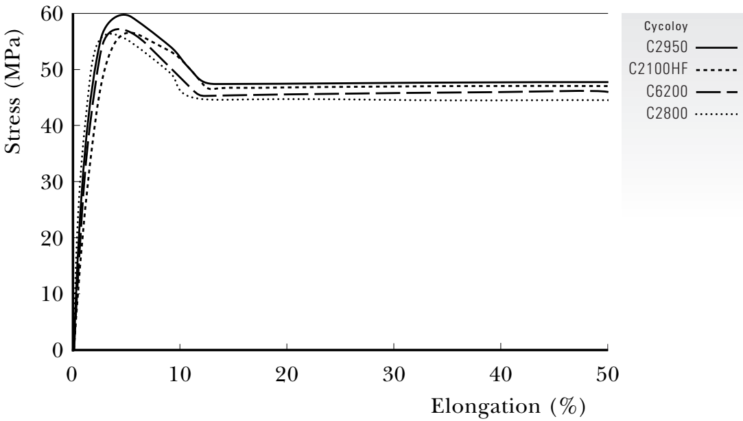
■ FIGURE 2 Stress-strain curve of flame retarded Cycloy at room temperature
