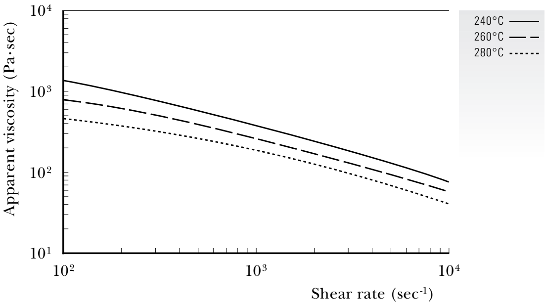
■ FIGURE 24 Capillary melt viscosity of Cicoloy C1100HF (DIN 54811)
