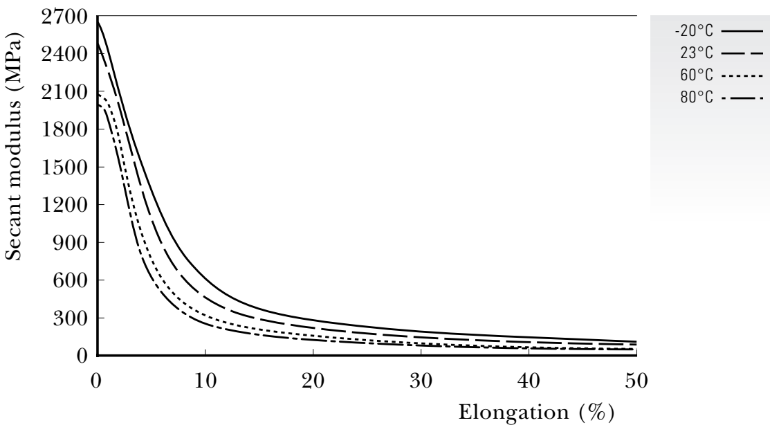
■ FIGURE 3 Secant modulus curve of Cycloy C1100HF
